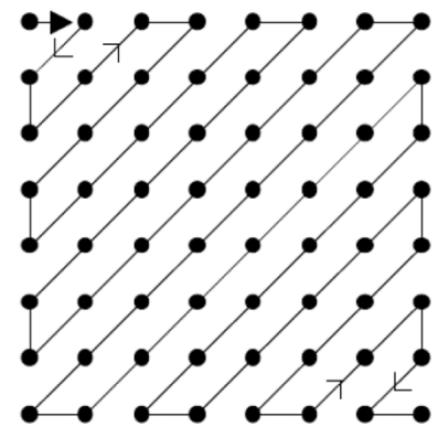
Figure - 6 (JPEG_naive.mlx)
