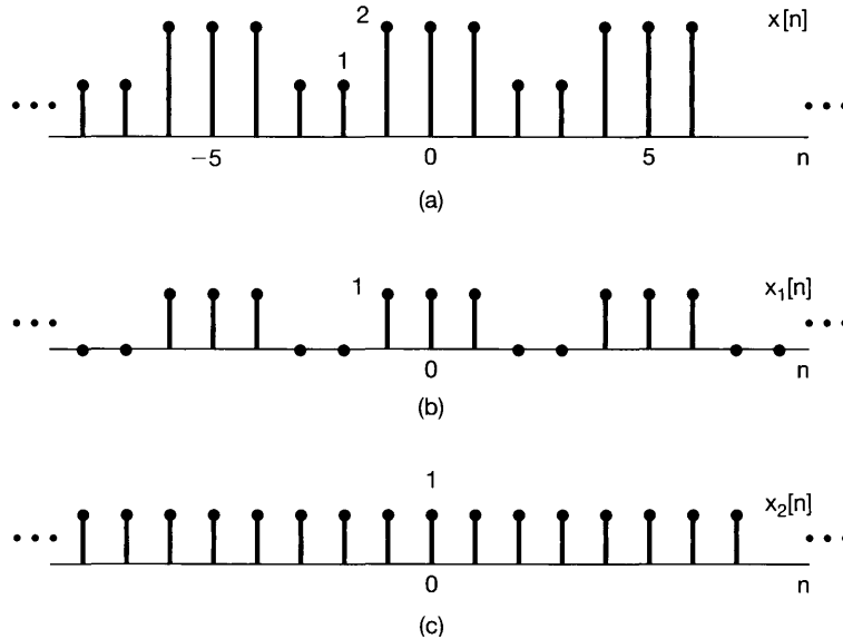
Figure 3.19 (a) Periodic sequence x[n] for Example 3.13 and its representation as a sum of (b) the square wave x_1[n] and (c) the dc sequence x_2[n] .
