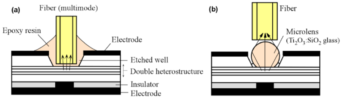
Figure 2: Coupling of light from LEDs into optical fiber
