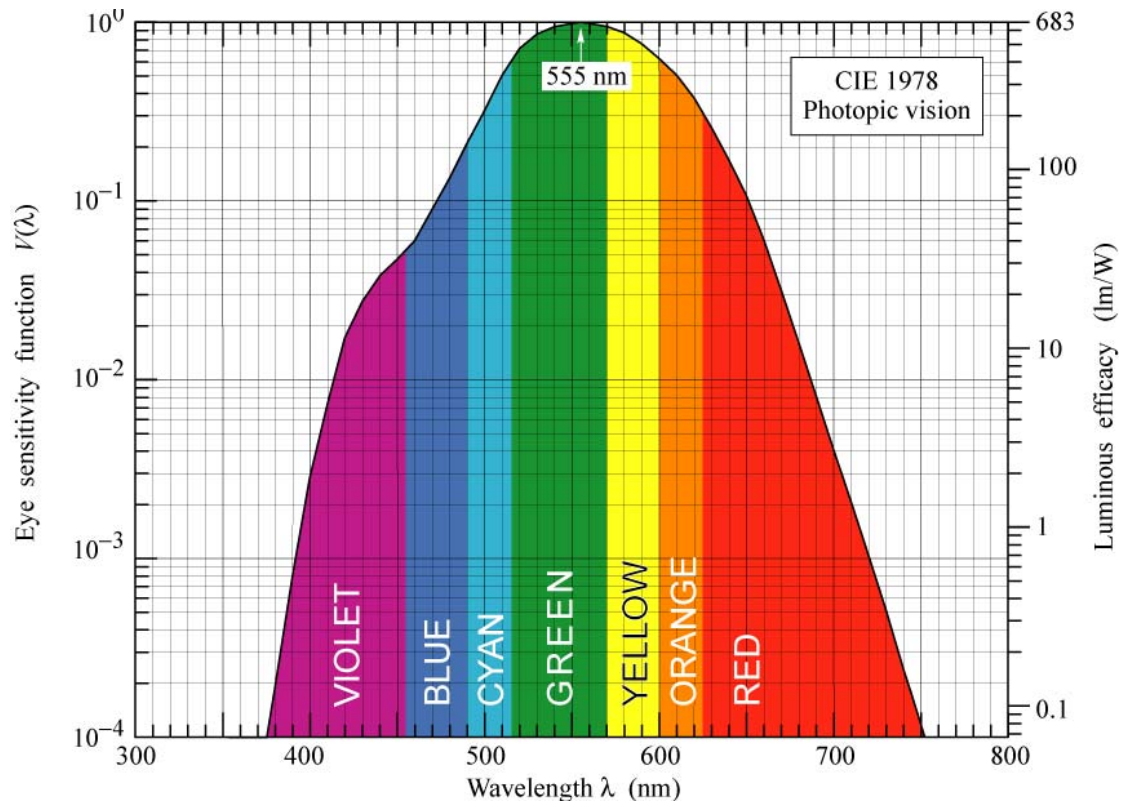
Figure 4: Visibility function V(\lambda) v.s. wavelength
