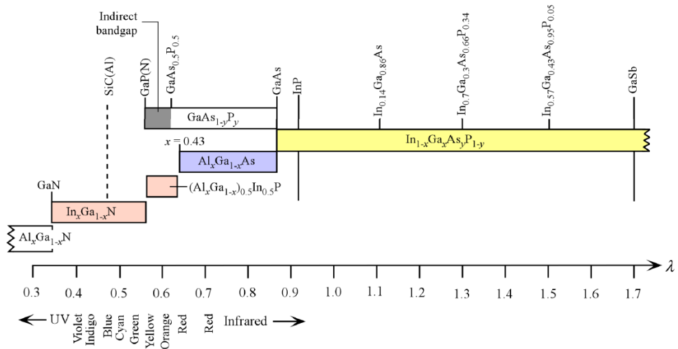
Figure 1: Emission wavelength v.s. LED materials
