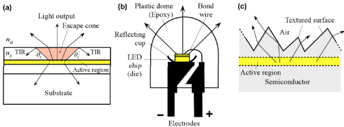
Figure 3: LED light extraction
